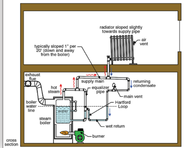
One pipe parallel flow system
