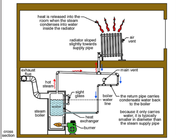
How steam systems work
