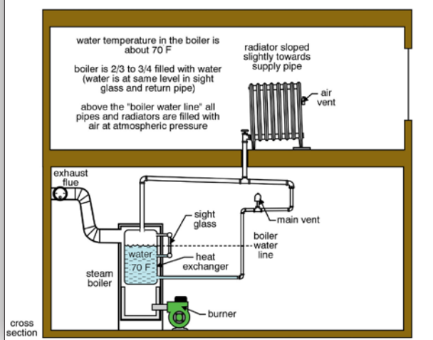
Steam system operation: at rest
