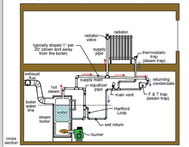
Two pipe system
